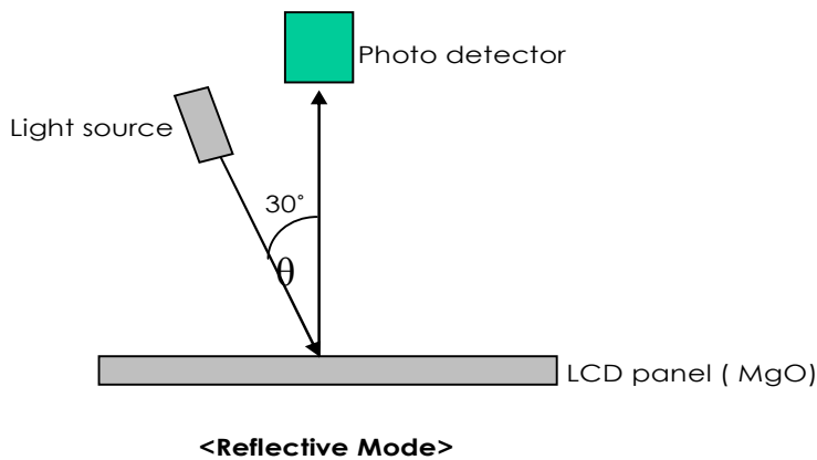
FIG. 4 Measuring method for optical characteristics in Reflective mode
