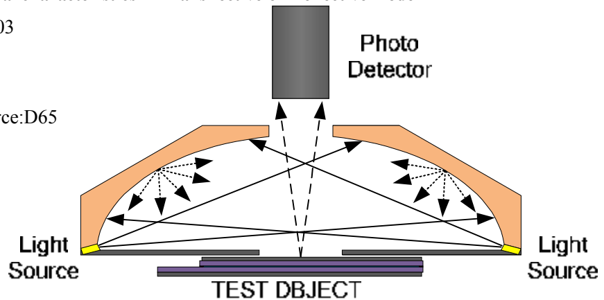
FIG.4. Measuring method for optical characteristics in Transflective or Reflective mode
